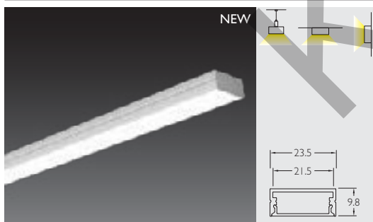
3198 Al Profile with PC Opal Matte Diffuser 4ft
