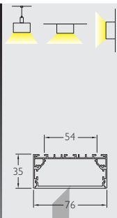
3087 Al Profile with PC Opal Matt Diffuser 1m / 4ft
