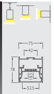
3085 Al Profile with PC Opal Matt Diffuser 1m / 4ft
