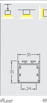
3197 Al Profile with PC Opal Matte Diffuser 4ft
