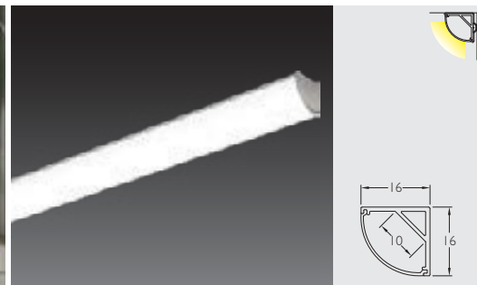
3084 Al Profile with PC Clear / Opal Matte Diffuser 1m
