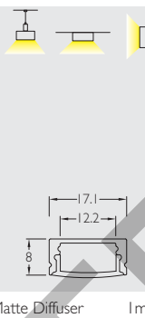
3225 Al Profile with PC Clear / Semi Clear Matte Diffuser 1m
