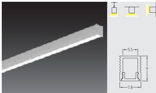
3196 Al Profile with PC Opal Diffuser 1m
