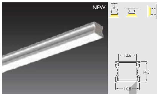
3227 Al Profile with PC Clear / Semi Clear Matte Diffuser 1m
