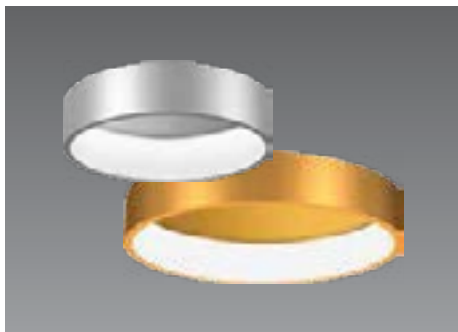
SHINE MIDI / SHINE Colour : Silver / Gold 3038 27W LED Ø450 x 126 3039 36W LED Ø598 x 126
